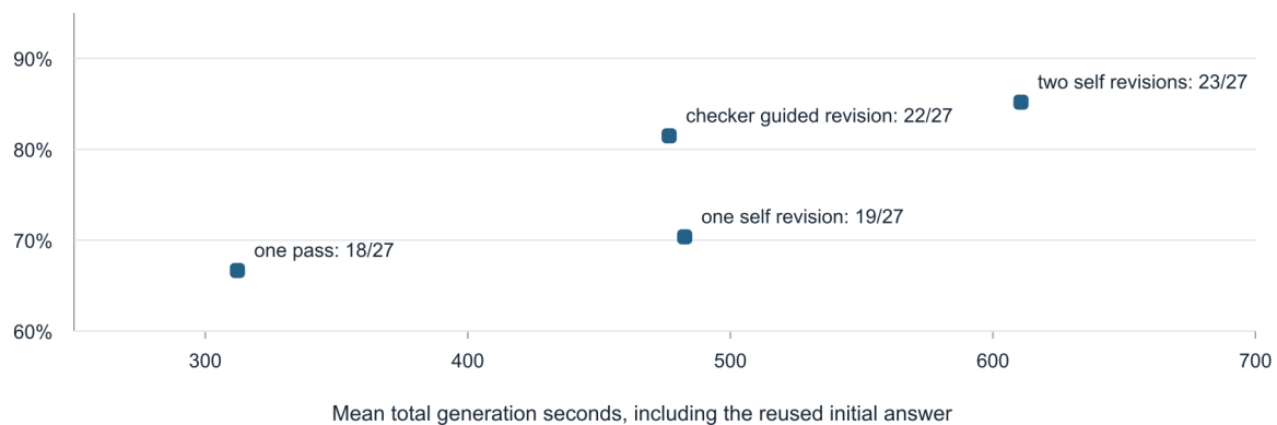
Figure 8: Revision accuracy against mean cumulative generation time. All branches share the same initial answers. The checker intervenes only on initially incorrect outputs.
