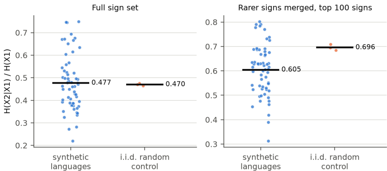
Figure 1. Plug-in conditional-to-unigram entropy ratio H(X2|X1)/H(X1) at the Indus point (2,906 texts, mean 4.6 signs; full calibration, seeds 0-2): full sign set (left) and rarer signs merged, top 100 signs (right). Dots are corpora (60 synthetic-language corpora, 3 i.i.d. random-control corpora); bars are means. Score label: not applicable, since Task A uses no reference language.
