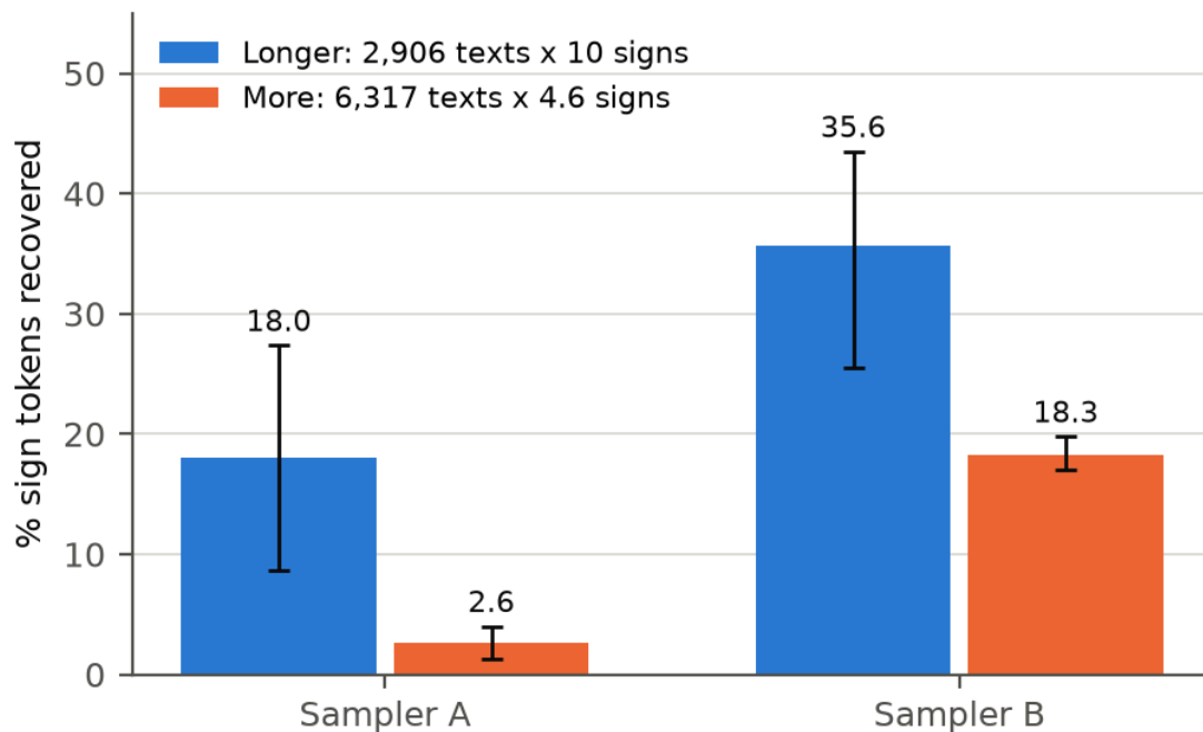
Figure 2. Longer vs more inscriptions at equal total tokens (about 29,000), candidates tier, original rule, both generators (sampler A = generator v1, sampler B = generator v2). Score label: primary (sister-v2, before the cognate step). Bars are means over 60 corpora; whiskers are 95% intervals resampling whole source languages.
