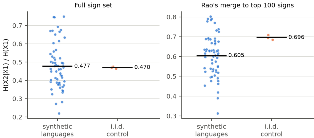
Figure 3. Entropy ratio H(X2|X1)/H(X1) at the Indus point (2,906 texts, mean 4.6 signs; full calibration, seeds 0-2), left on the full sign set, right after Rao's merge to the 100 most frequent signs. Dots are corpora (60 synthetic-language corpora, 3 i.i.d.-control corpora); bars are means. Score label: not applicable; Task A uses no reference language, so no sister or cognate step is involved.
