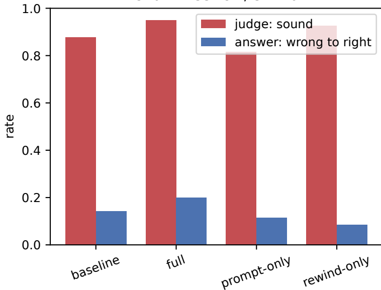
Mistral-7B GSM8K / Sinkhorn
