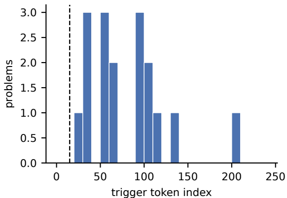
Qwen2.5 GSM8K Sinkhorn (n=17)
