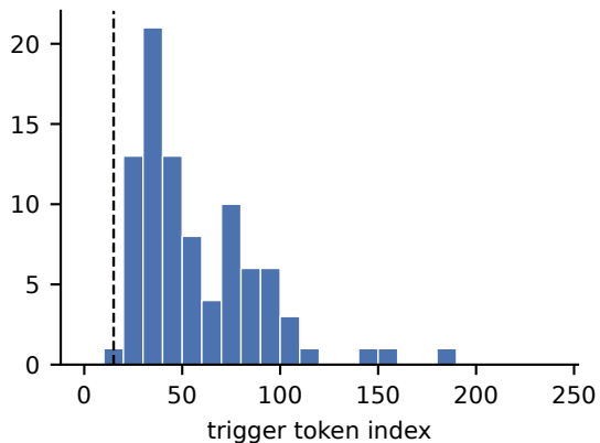
Qwen2.5 SVAMP Sinkhorn (n=89)
