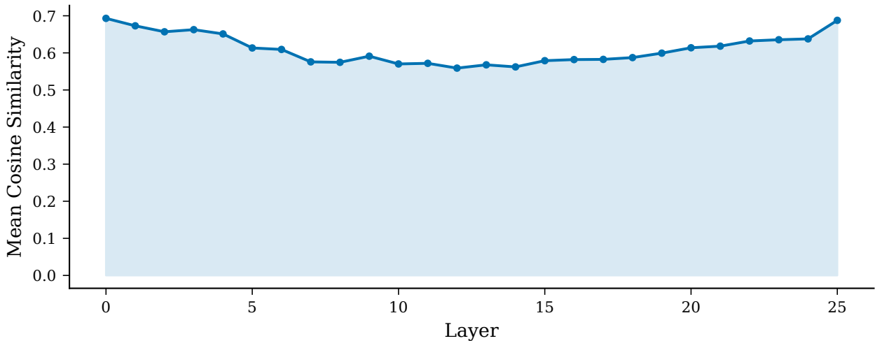
Dispersion Profile: Refusal — gemma-2-2b-it
