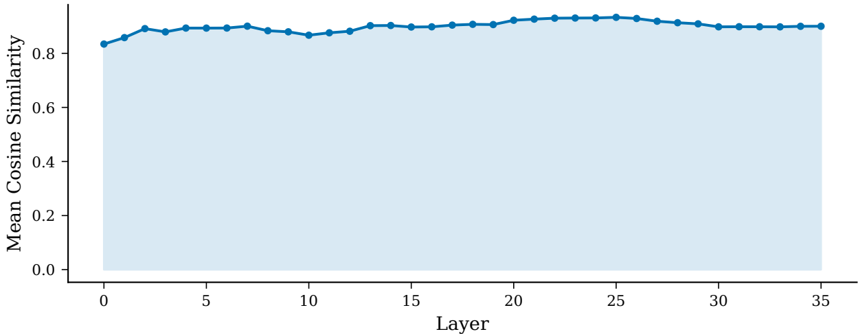
Dispersion Profile: Refusal — qwen-2.5-3b
