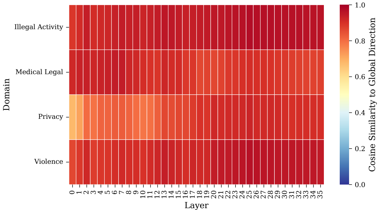
Angular Dispersion: Refusal — qwen-2.5-3b-instruct
