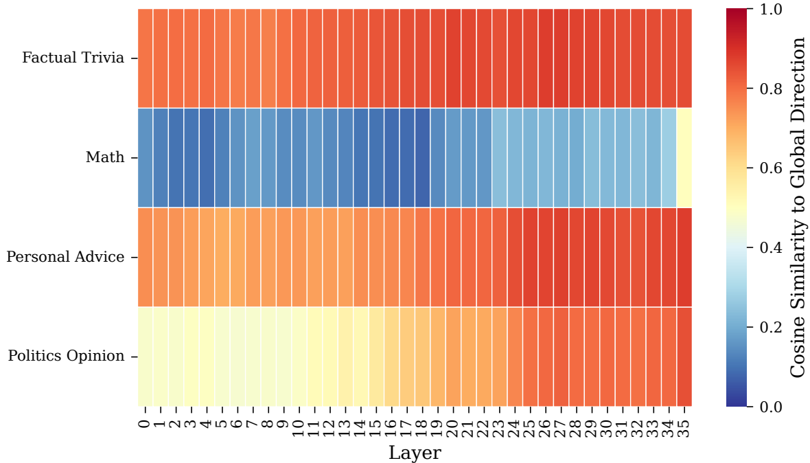
Angular Dispersion: Honesty — qwen-2.5-3b-instruct
