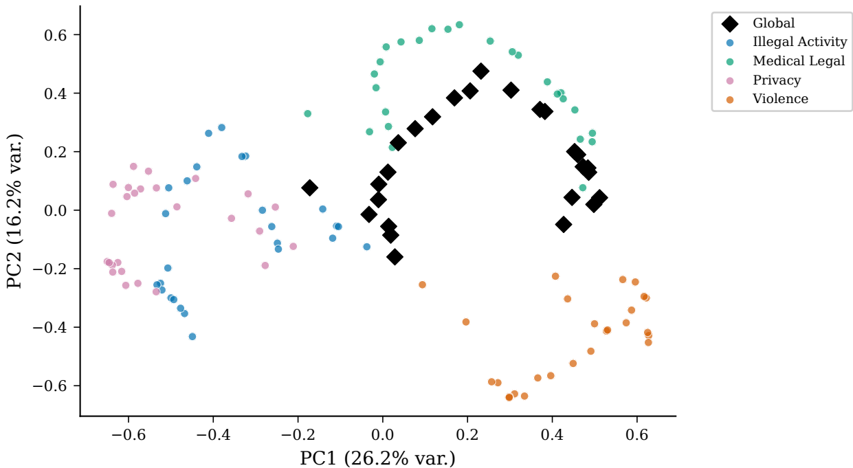
Direction Geometry: Refusal — gemma-2-2b
