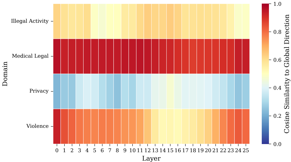
Angular Dispersion: Refusal — gemma-2-2b
