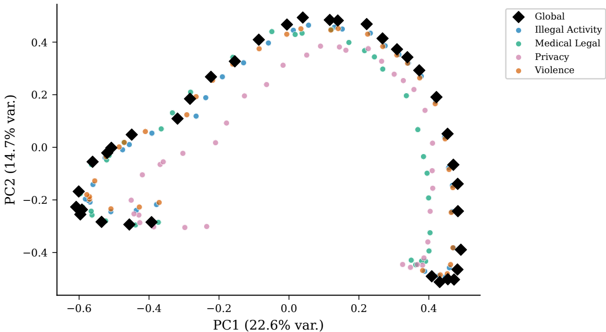
Direction Geometry: Refusal — qwen-2.5-3b
