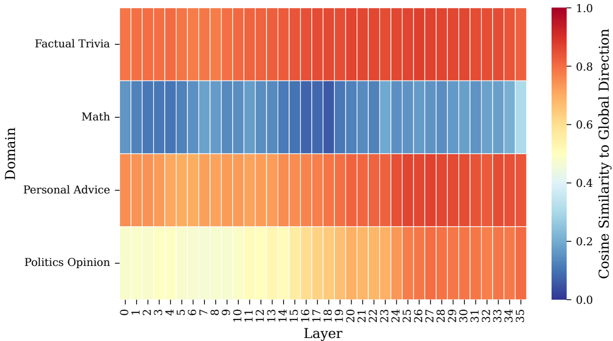
Angular Dispersion: Honesty — qwen-2.5-3b
