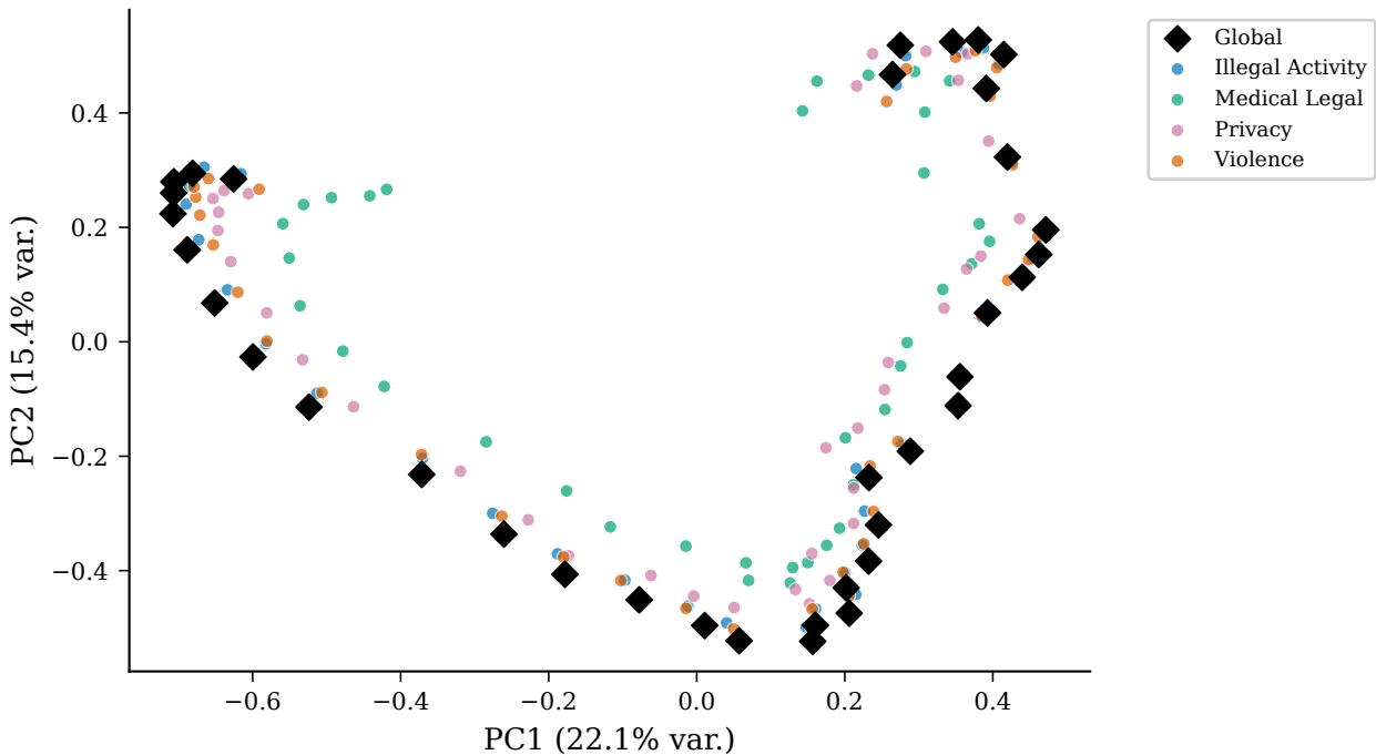
Direction Geometry: Refusal — qwen-2.5-3b-instruct
