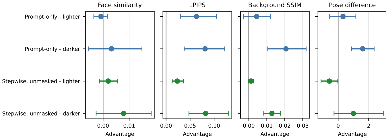
Preservation at matched +/-5 ITA change (mean paired advantage, 95% CI)
