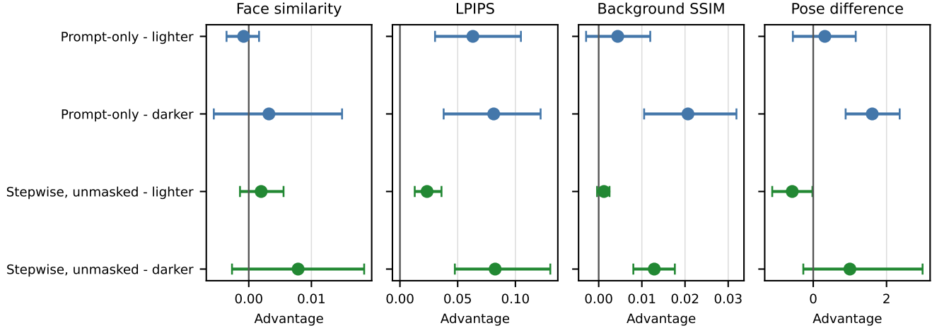
Preservation at matched \pm 5 ITA change (mean paired advantage, 95% CI)
