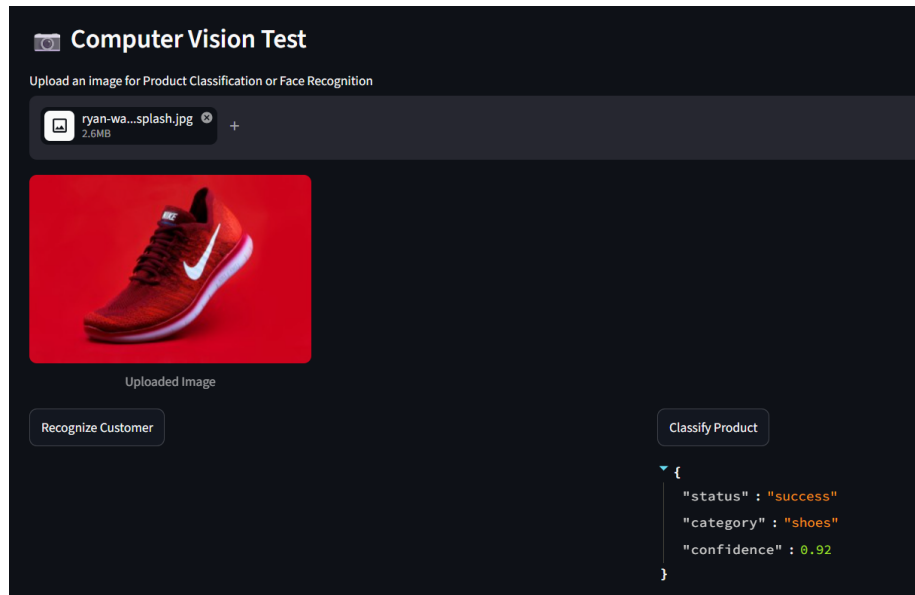
Figure 5: Product Image Classification and Computer Vision Interface
