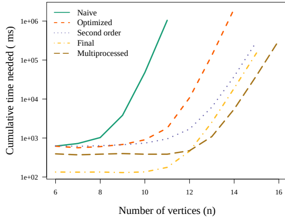
Figure 1: A comparison between different versions of the algorithm, tested on all planar triangulations for a given number of vertices. The naive algorithm is the simplest algorithm described in Algorithm 5. Optimized is the implementation that has implemented the available colors, permutations and bit-sets optimizations. The second order implementation has also implemented the updating of neighbors' neighbors. Lastly, the final and multithreaded implementations are the final C implementation and its multithreaded version using 10 processes respectively. Each implementation performs better than the last.
