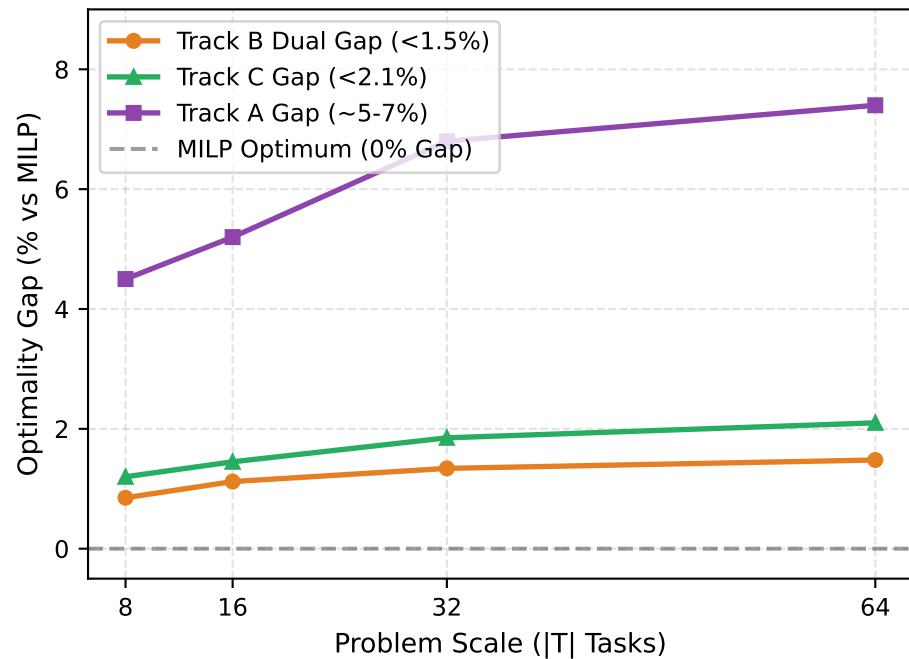
(b) Solution Quality vs Scale
