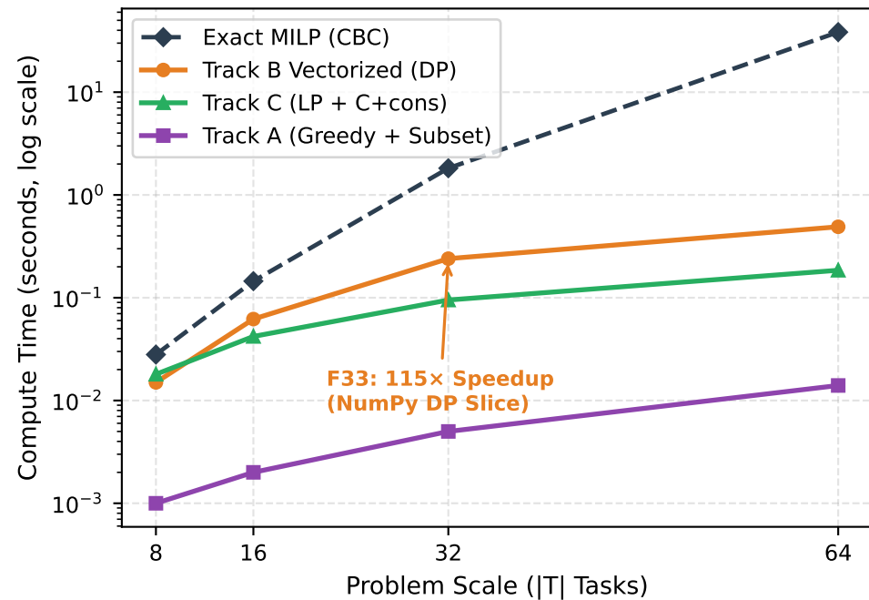
(a) Solver Runtime vs Scale
