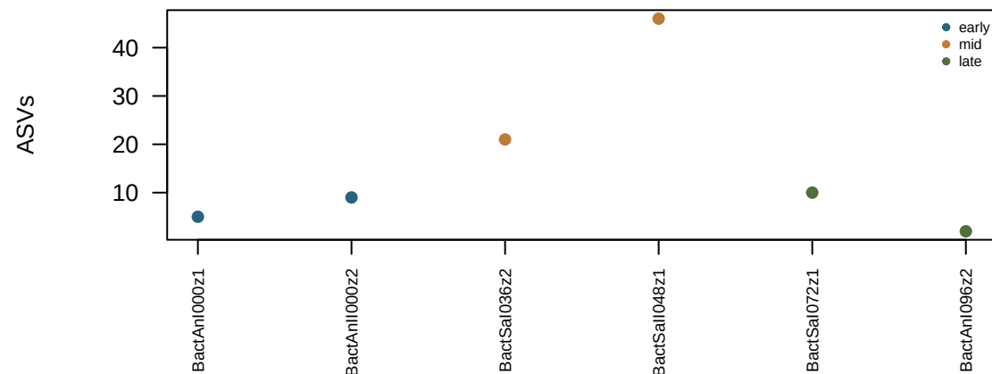
Observed ASVs
