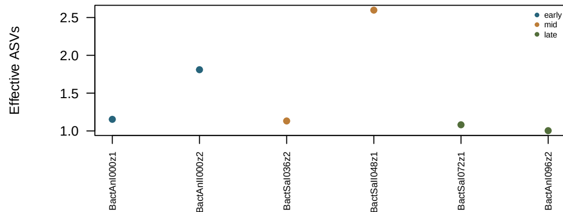
Inverse Simpson
