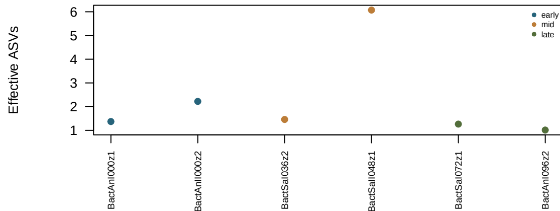
Shannon effective diversity
