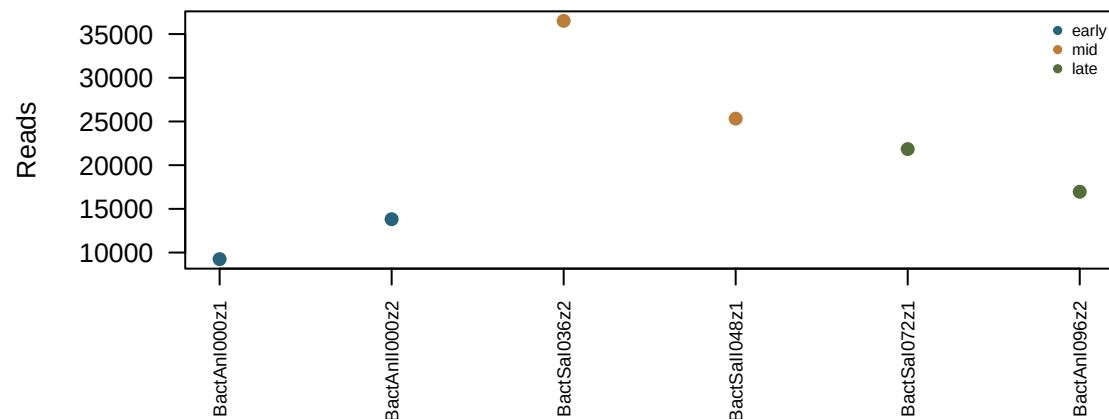
Retained reads
