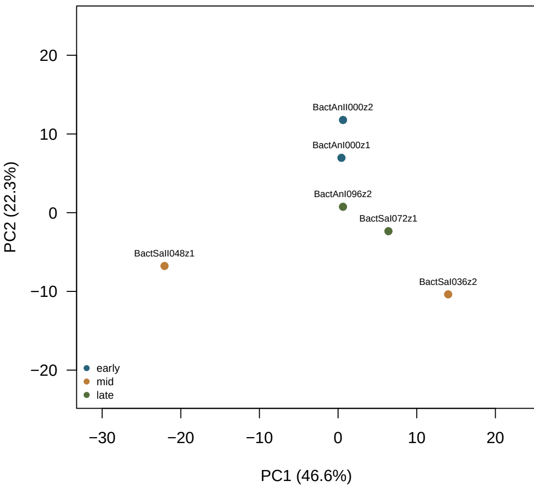
CLR PCA Count pseudocount = 1
