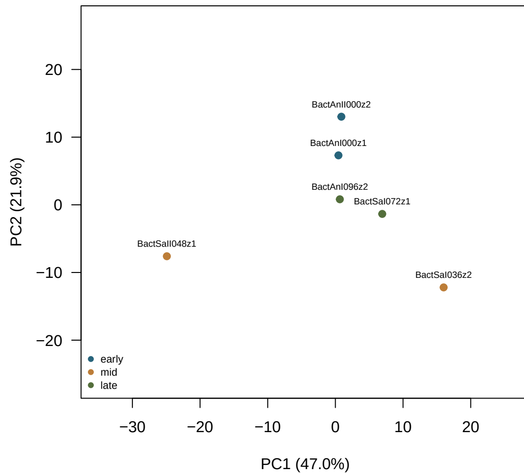
CLR PCA Count pseudocount = 0.5
