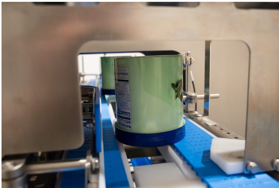
Inside the inspection tunnel: a tub rides the two independent belts past the sidewall code reader.
