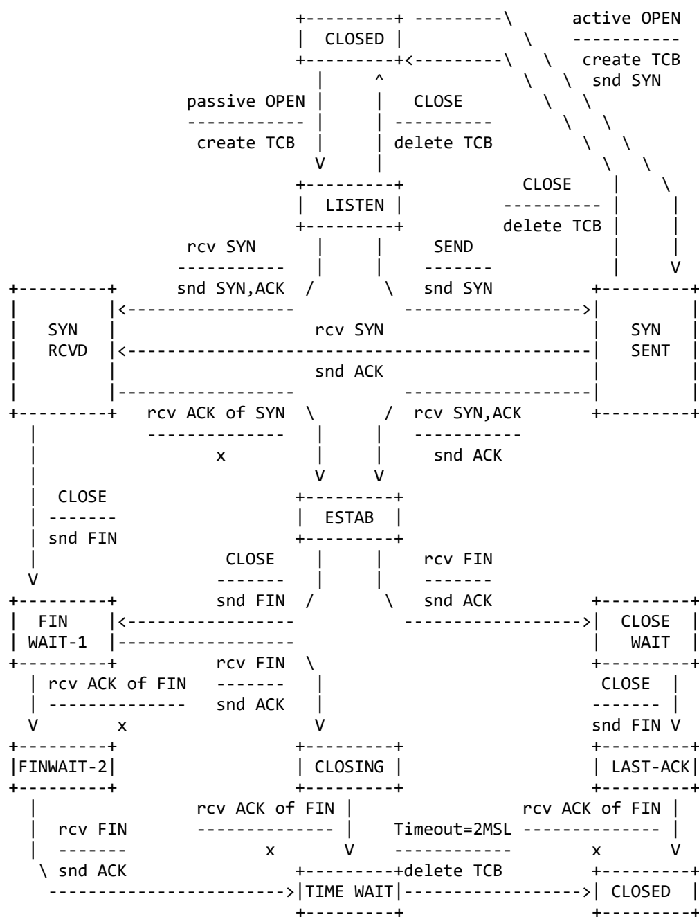
TCP Connection State Diagram Figure 6.
