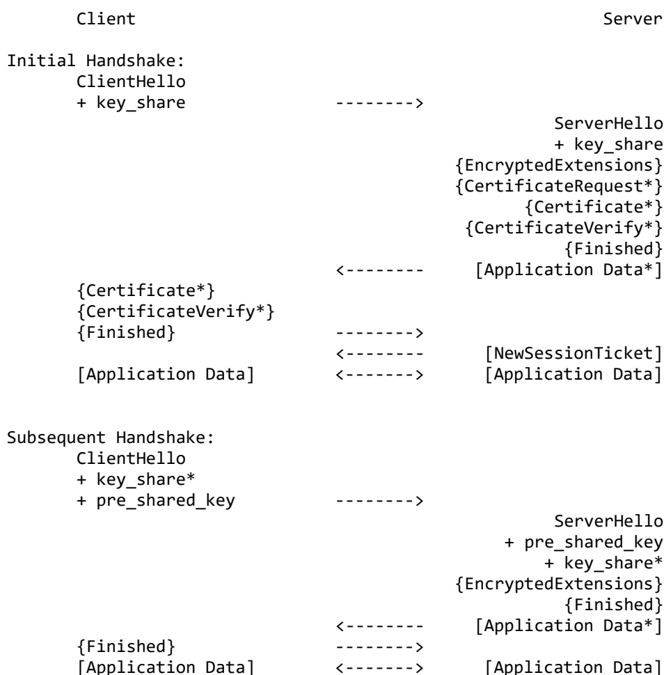
Figure 3: Message Flow for Resumption and PSK
