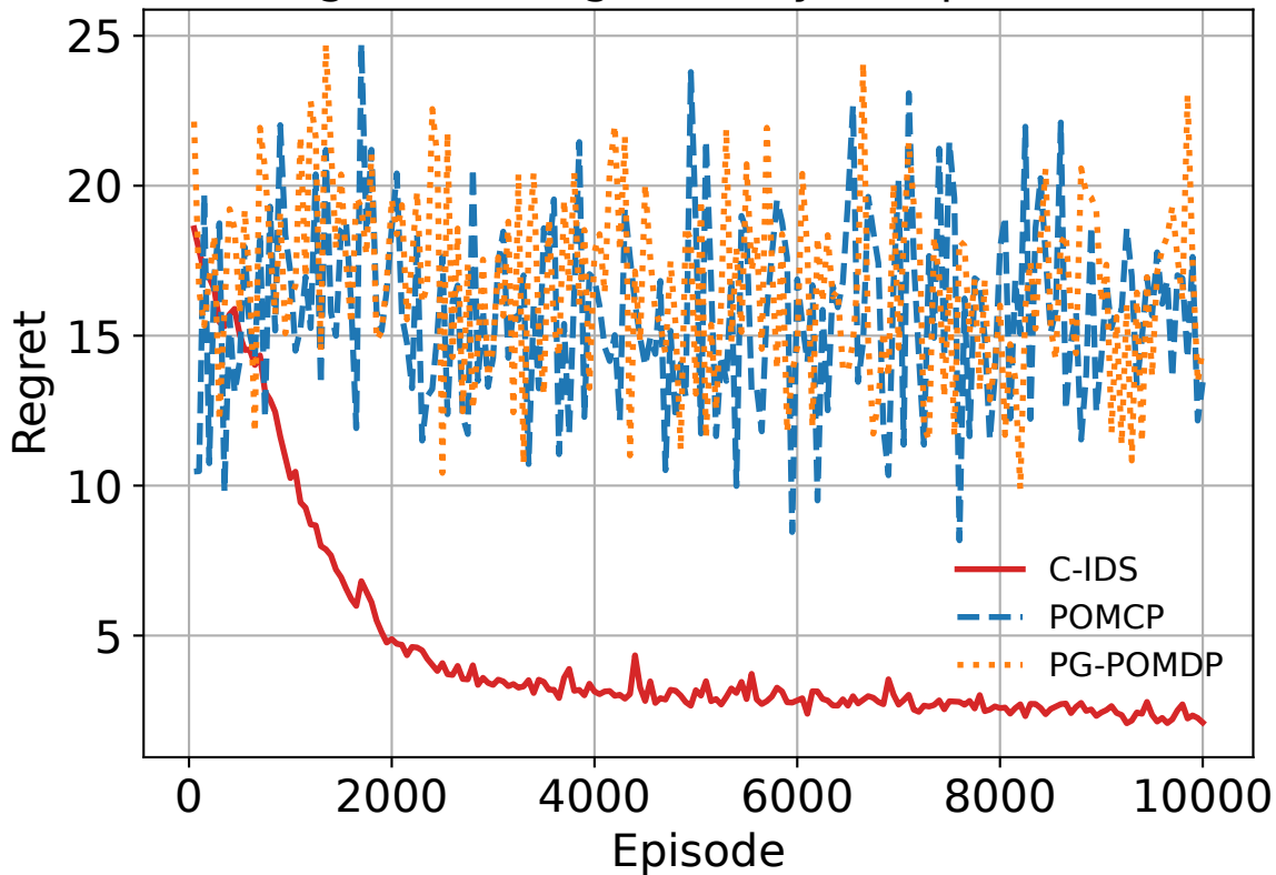
Regret (averaged every 50 episodes)
