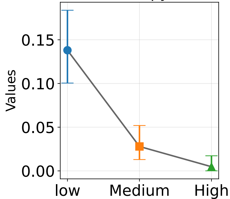
Entropy
