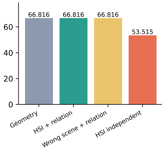
Contact (%) ↑
