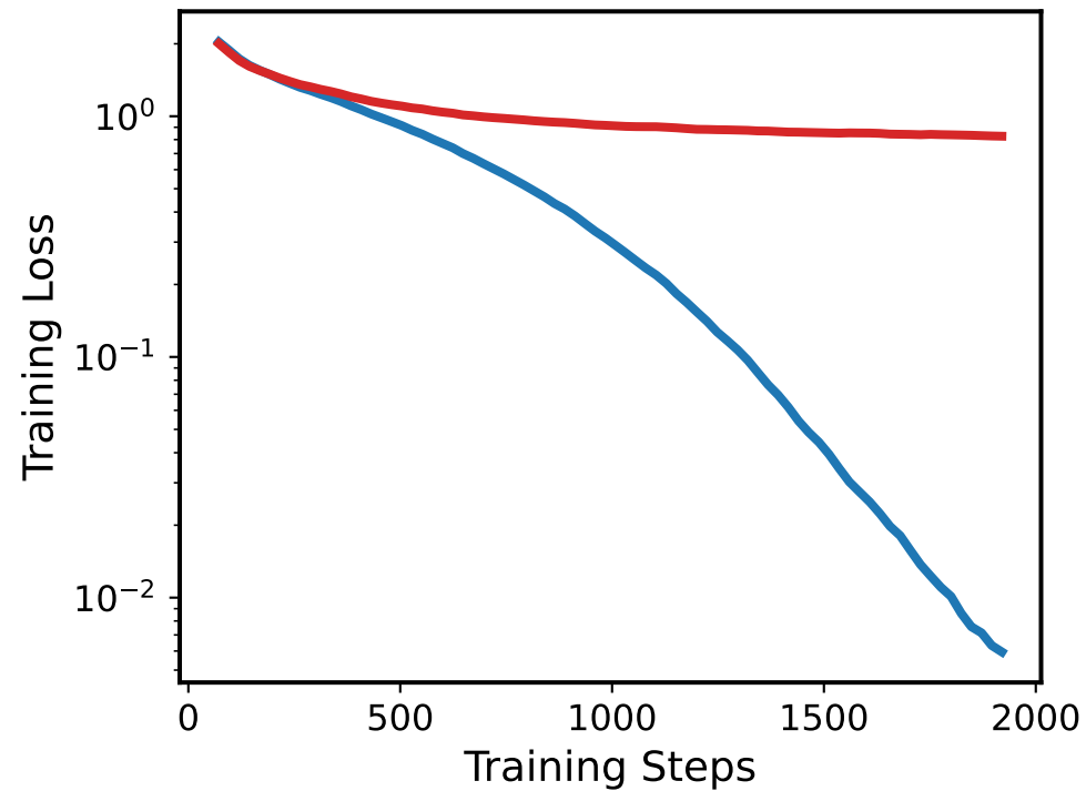
Training Loss
