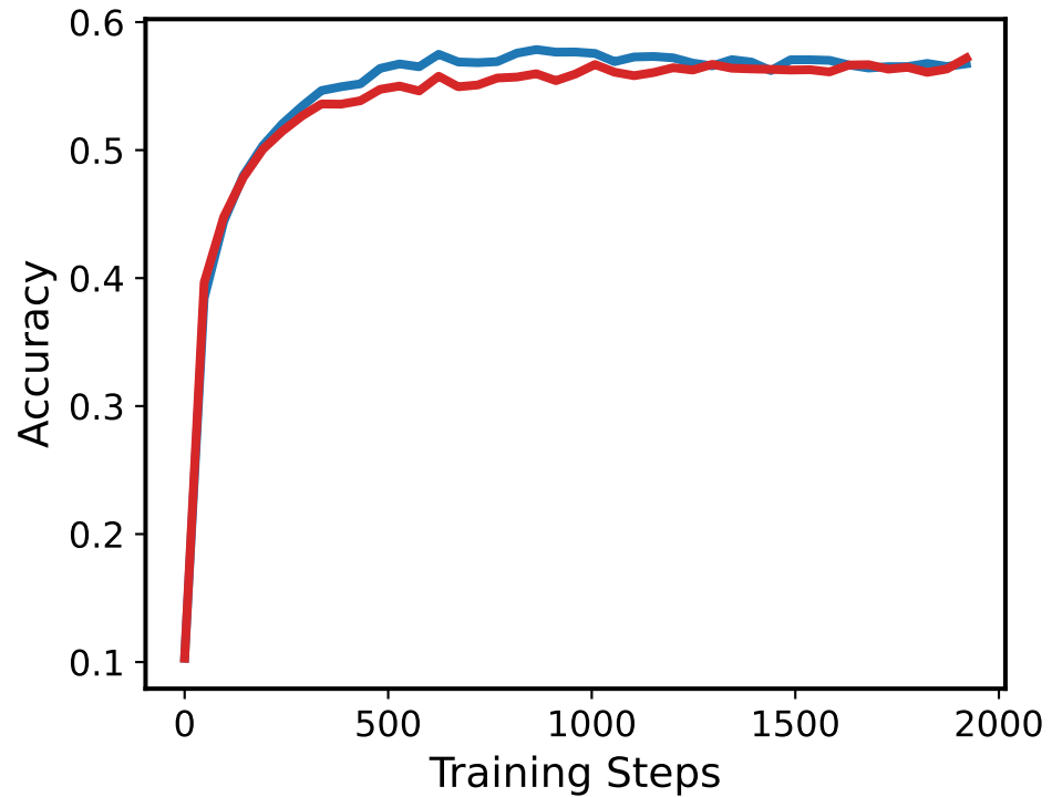
Test Accuracy
