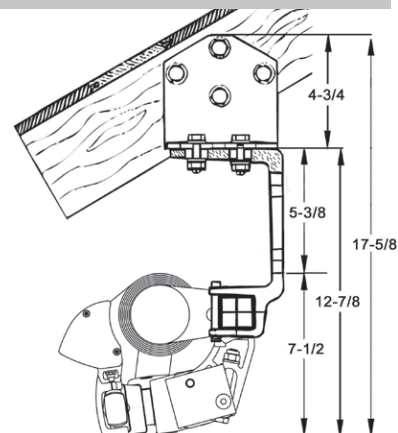
Sunstyle Rafter Bracket With Universal Bracket
