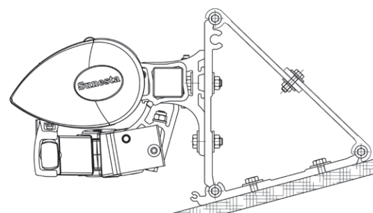
Sunstyle Roof Bracket Kit With SmartCase™
