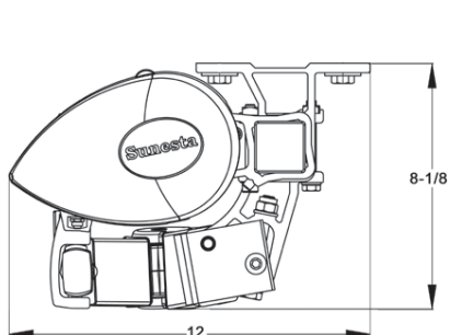
Sunstyle Ceiling Bracket Kit With SmartCase™
