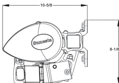
Sunstyle Wall Bracket Kit With SmartCase™
