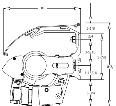
Sunstyle Wall Bracket With Hood
