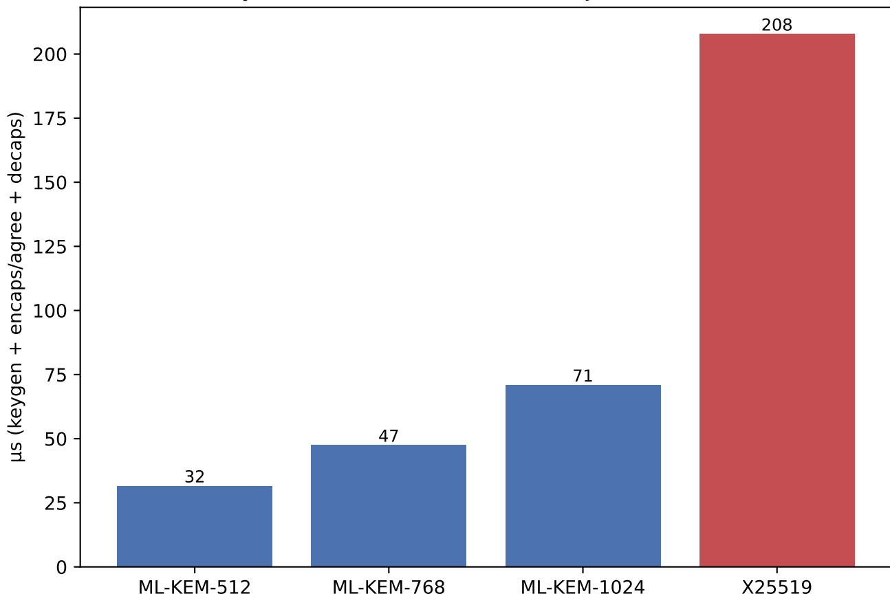
Key establishment cost: ML-KEM (JDK) vs X25519
