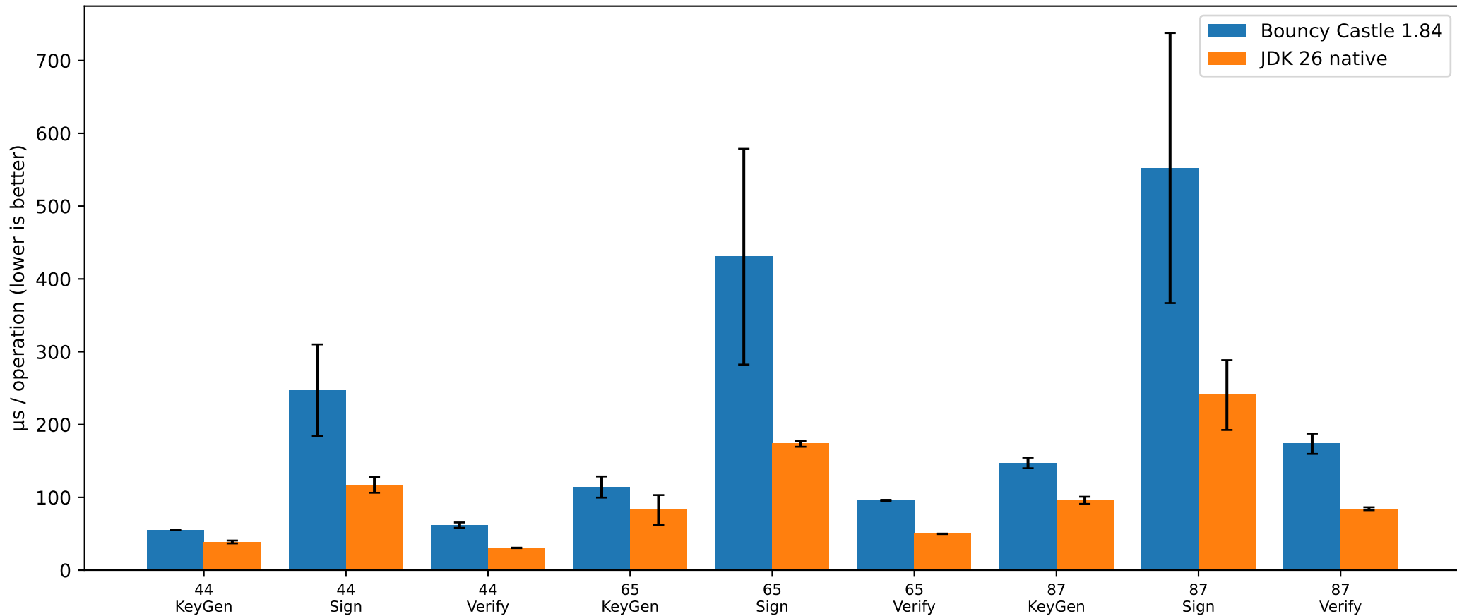
ML-DSA: Bouncy Castle 1.84 vs JDK native
