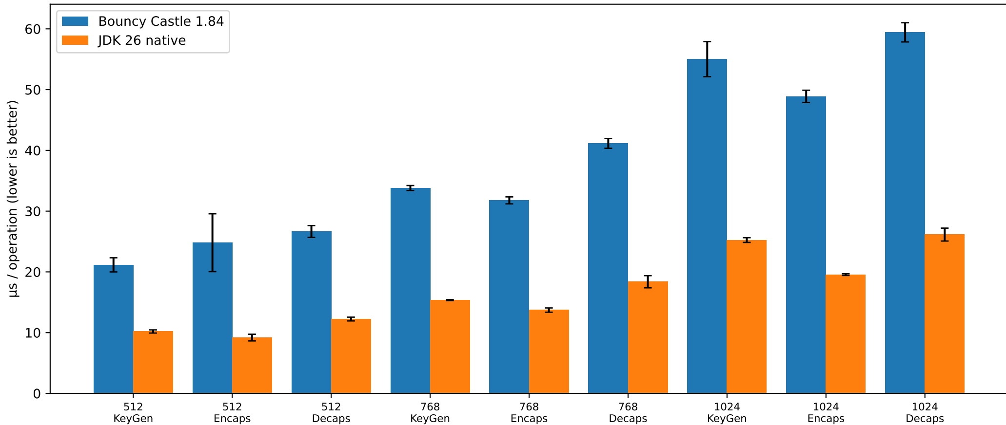
ML-KEM: Bouncy Castle vs JDK native
