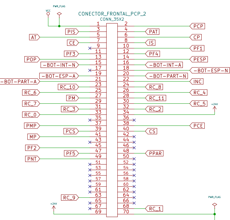
CONECTOR FRONTAL
