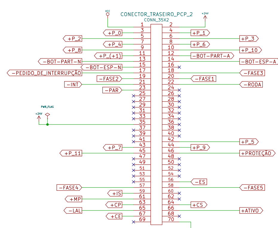
PCP-2: PLAC "Debounce drivers para
