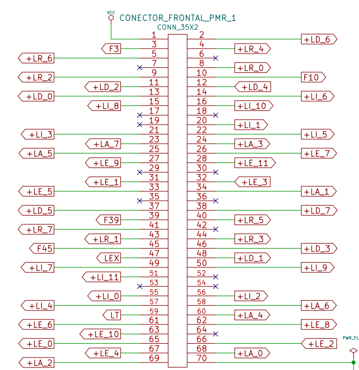
CONECTOR FRONTAL
