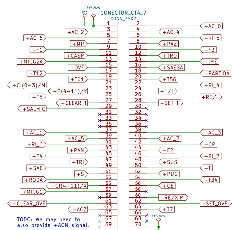
Placa CT4-7: Sinais de control
