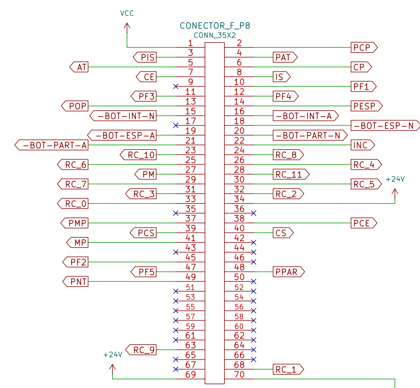
CONECTOR FRONTAL
