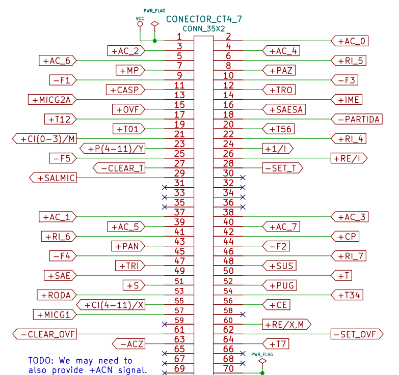
Placa CT4-7: Sinais de control
