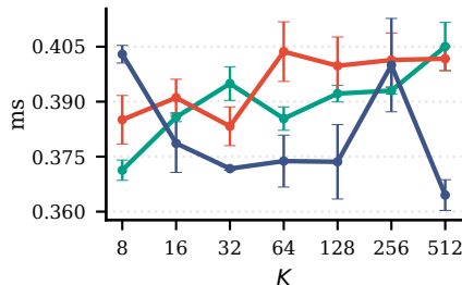
Segment: next_batch
