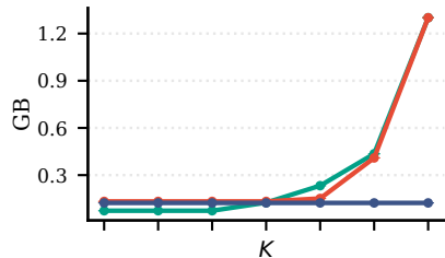
Segment: next_batch
