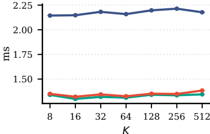
Profile: pair_slices
