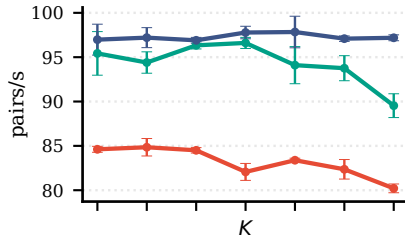
Profile: pair_slices
