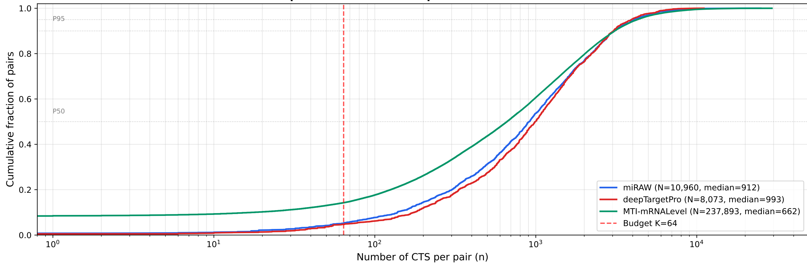
Empirical CDF: CTS Count per Pair Across Datasets
