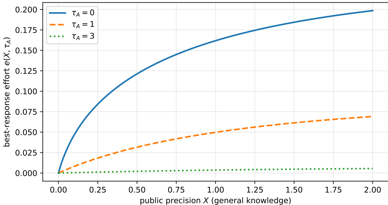
Observation 2: effort rises with X , falls with \tau_A ( \varepsilon = 2 )
