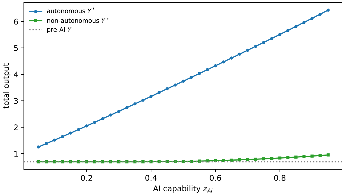
Output: autonomous > non-autonomous (Proposition 6.1)
