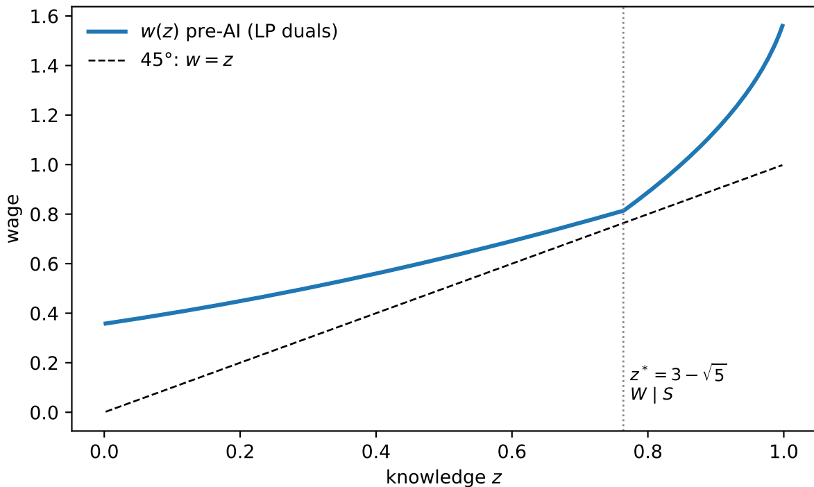
Pre-AI equilibrium, G(z) = z , h = 1/2 (paper's Figure 3a)
