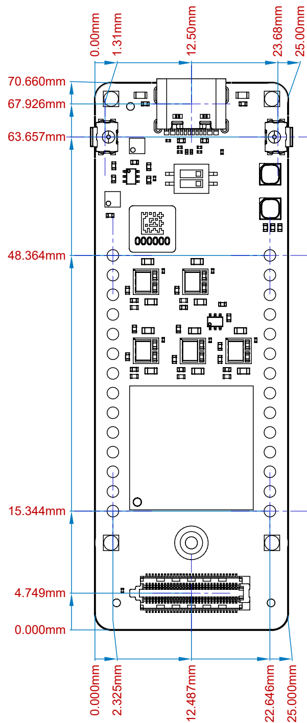
View from Top side (SDcale 2:1)
