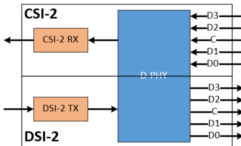
Figure 2-1 : MIPI Camera and Display components
