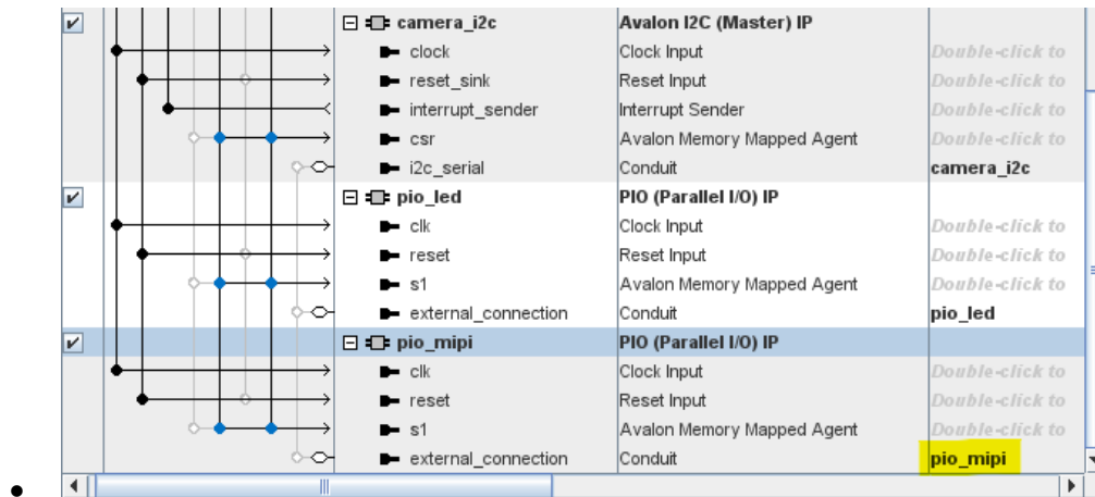
Figure 6-57: MIPI PIO connections
