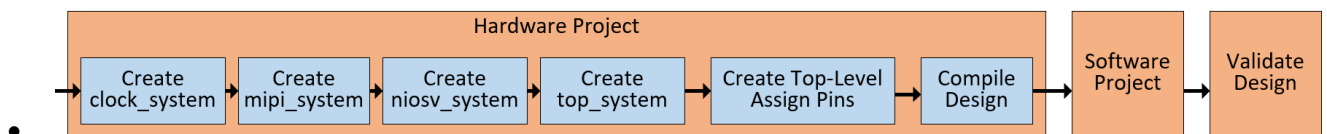
Figure 5-2 : MIPI Project Design Flow
