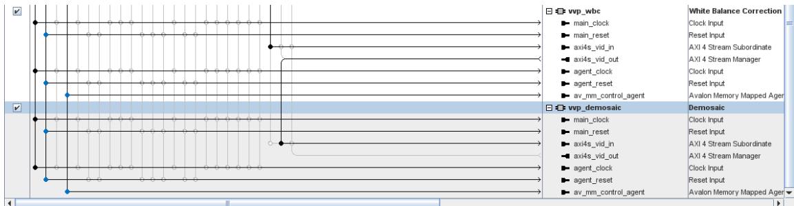
Figure 6-33: Demosaic Input connections
