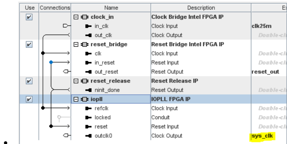
Figure 6-15: Add and connect IOPLL IP
