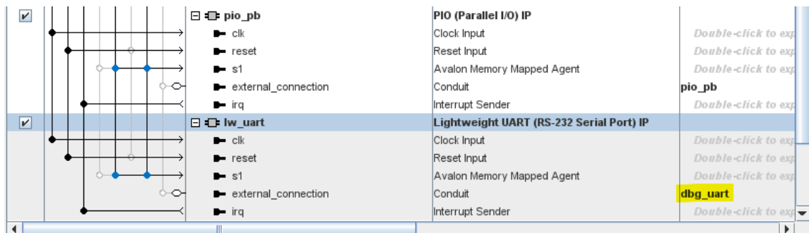
Figure 6-61: UART connections
