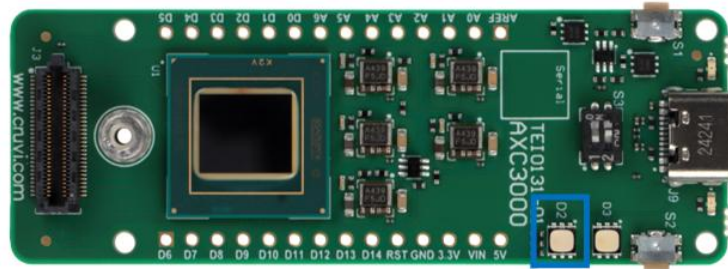
Figure 8-8 : LED D2 indicator
