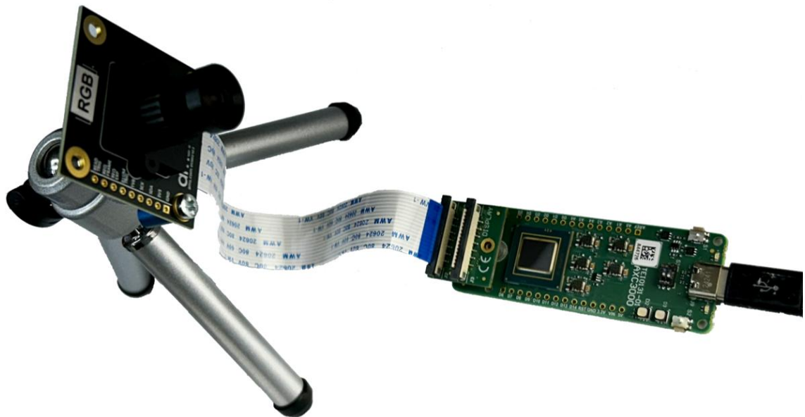
Figure 8-1 : Connected Hardware
