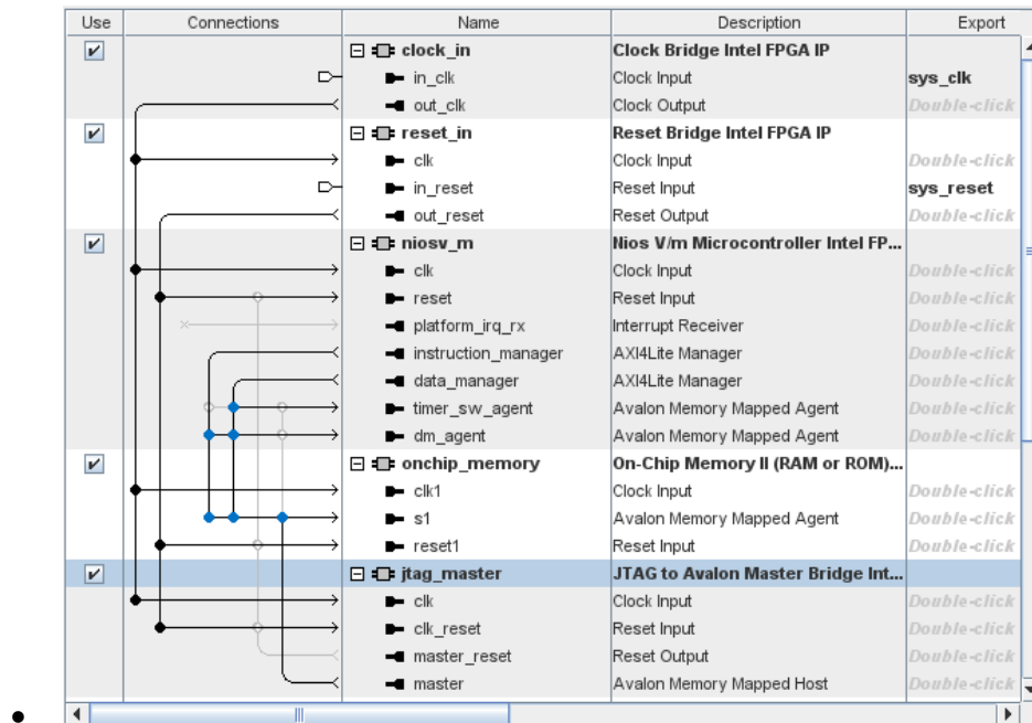
Figure 6-50: Add JTAG Avalon Master IP and connections
