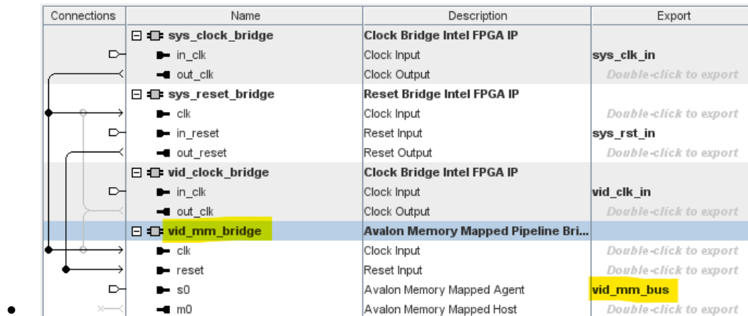
Figure 6-22: Connect Clock and Reset to MM Bridge
