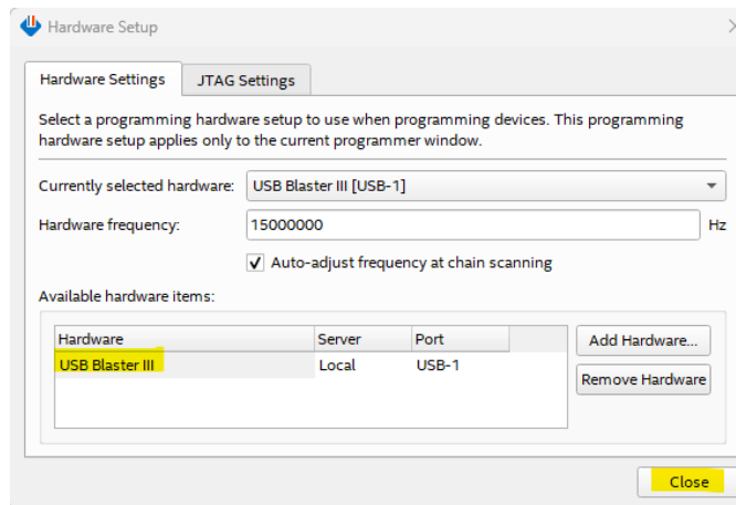
Figure 8-20 : USB Blaster Hardware Setup
