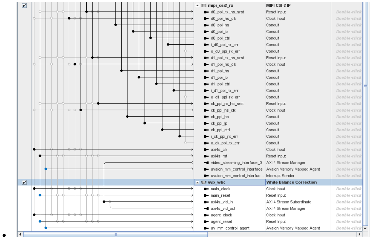
Figure 6-31: White Balance Correction connections
