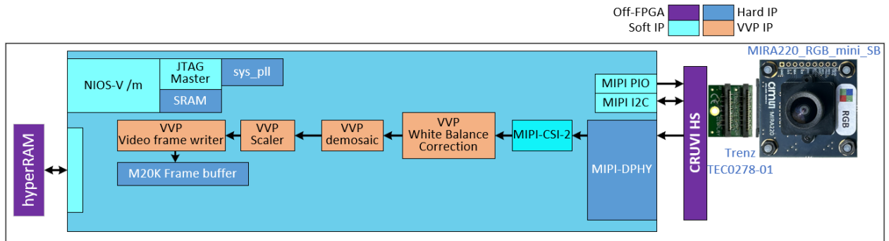
Figure 1-1 : Hardware Project Block Diagram
