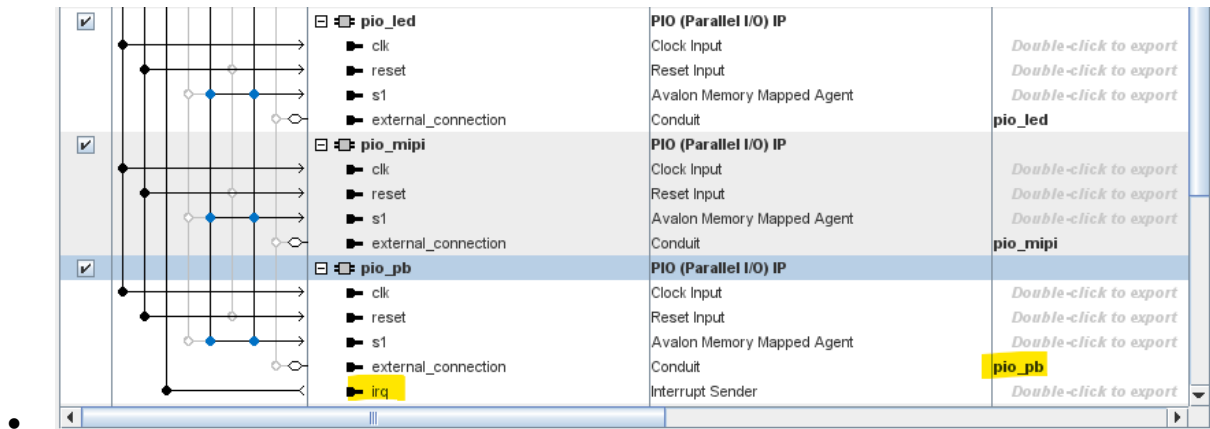
Figure 6-59: Push-Button PIO connections
