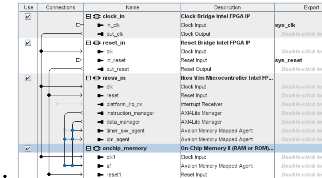
Figure 6-48: Onchip Memory connections
