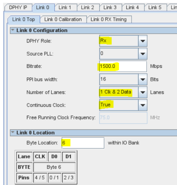
Figure 6-23: DPHY Link0 top-level settings
