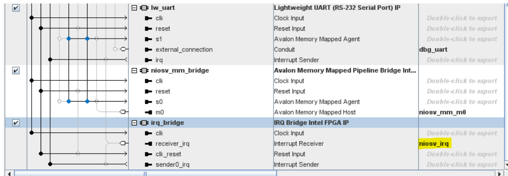
Figure 6-65: IRQ bridge connections
