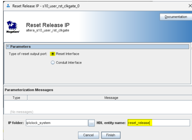
Figure 4-17 : Reset Release IP settings
