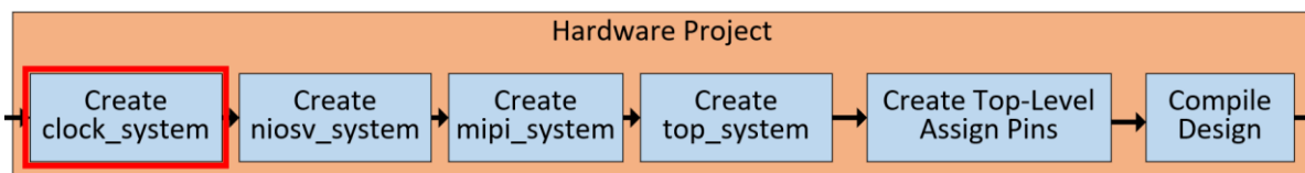
Figure 6-9: Create Clock/Reset subsystem
