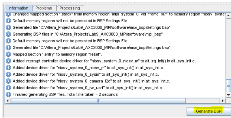
Figure 6-75: Generate BSP
