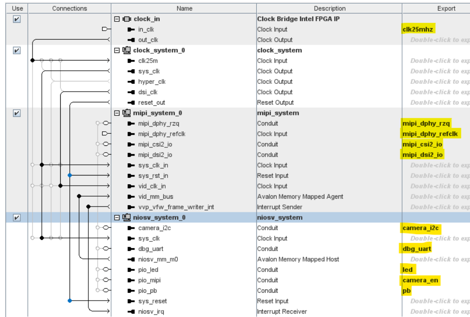
Figure 6-71: top_system connections
