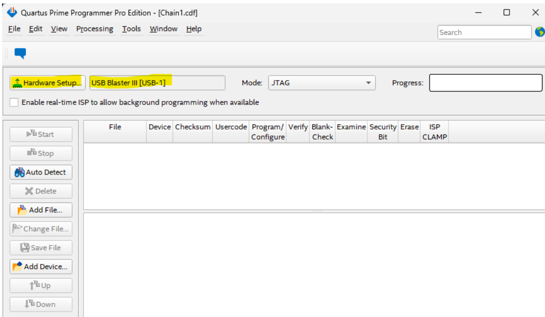
Figure 8-19 : Quartus Programmer
