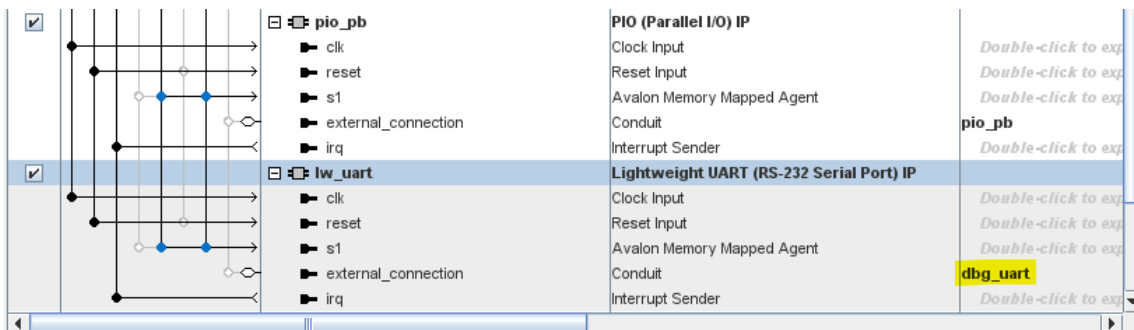
Figure 6-61: UART connections
