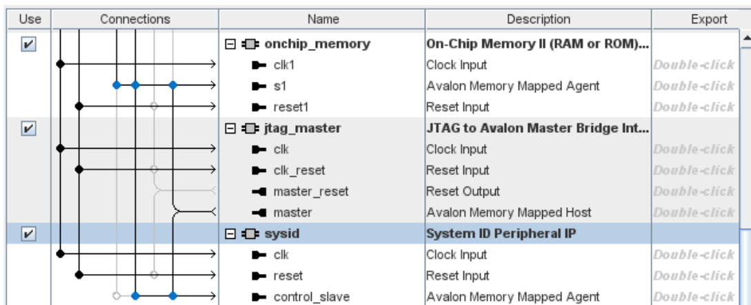
Figure 6-52: System ID connections
