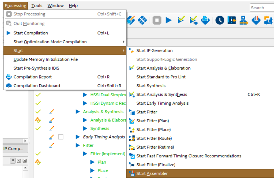
Figure 7-9 : re-run Assembler
