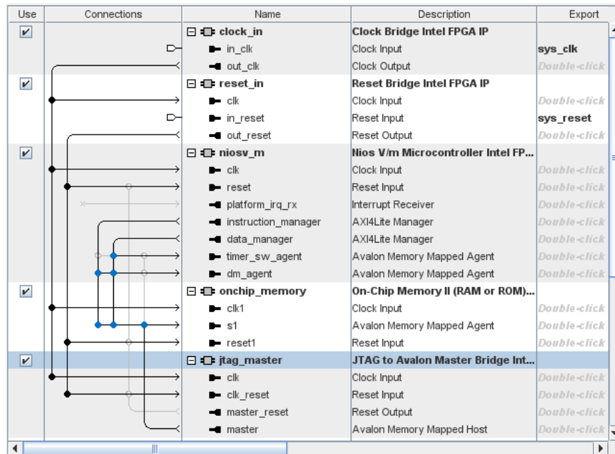
Figure 6-50: Add JTAG Avalon Master IP and connections
