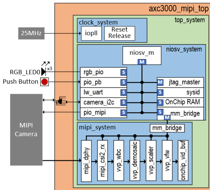
Figure 5-1: Project Block Diagram
