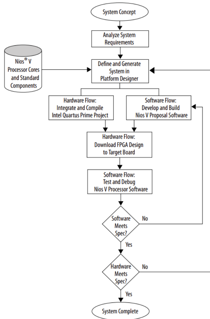
Figure 3-1 : Design Flow
