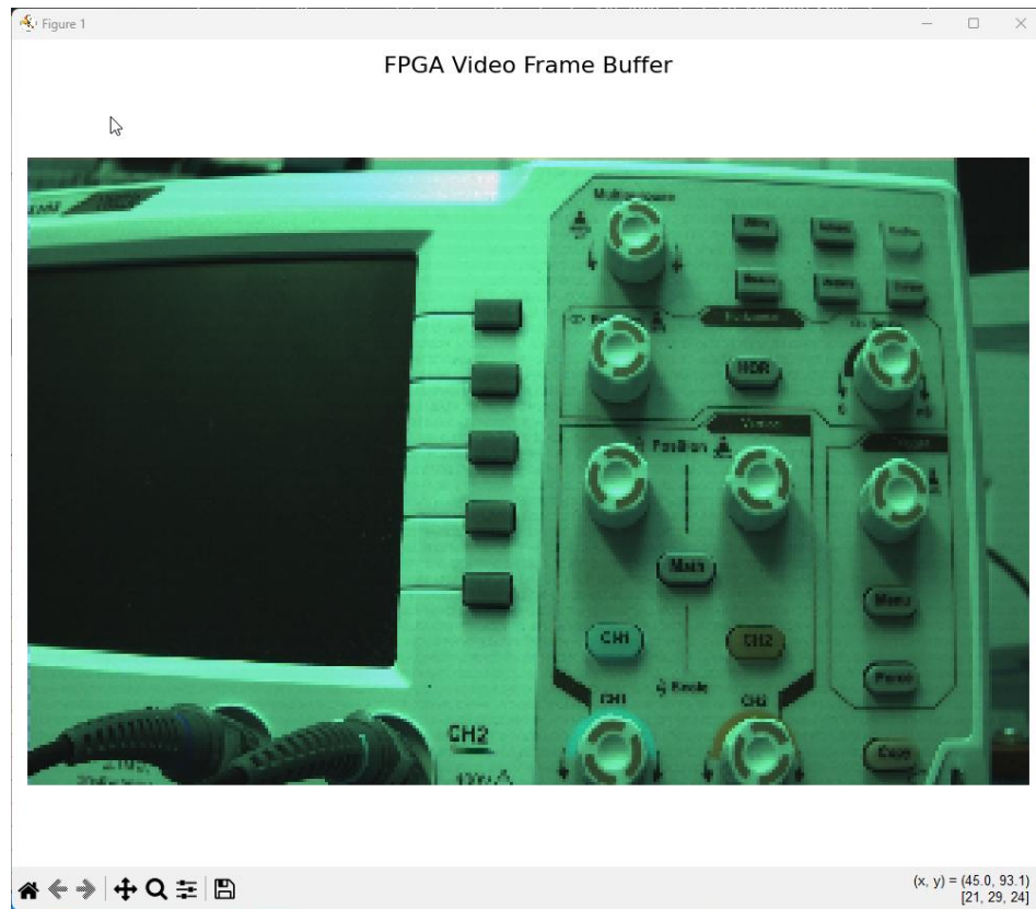
Figure 8-11: Image viewer
