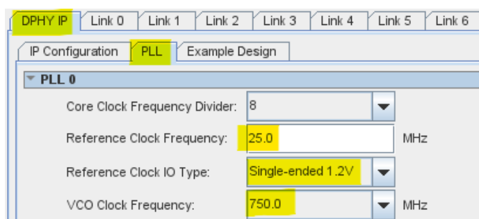
Figure 6-26: DPHY PLL settings
