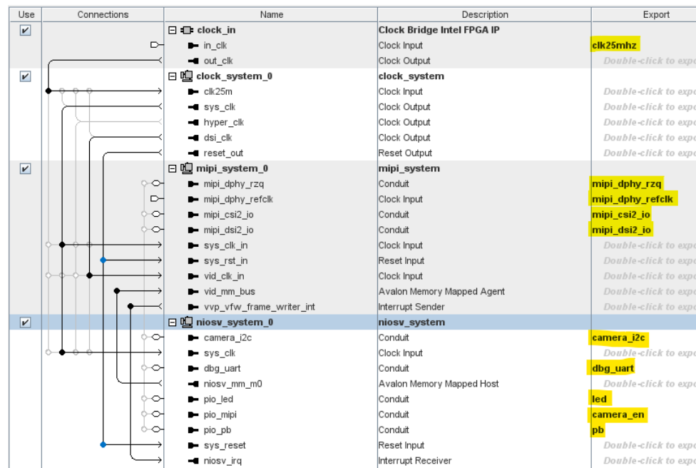
Figure 6-71: top_system connections
