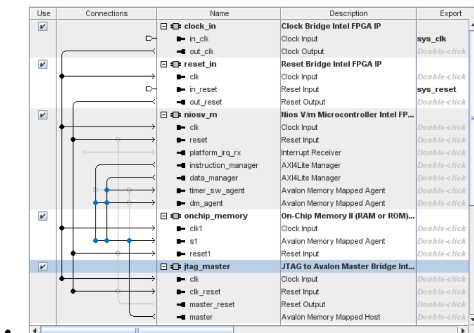
Figure 6-50: Add JTAG Avalon Master IP and connections
