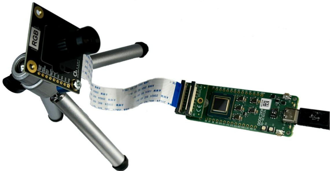
Figure 8-16 : Connected Hardware
