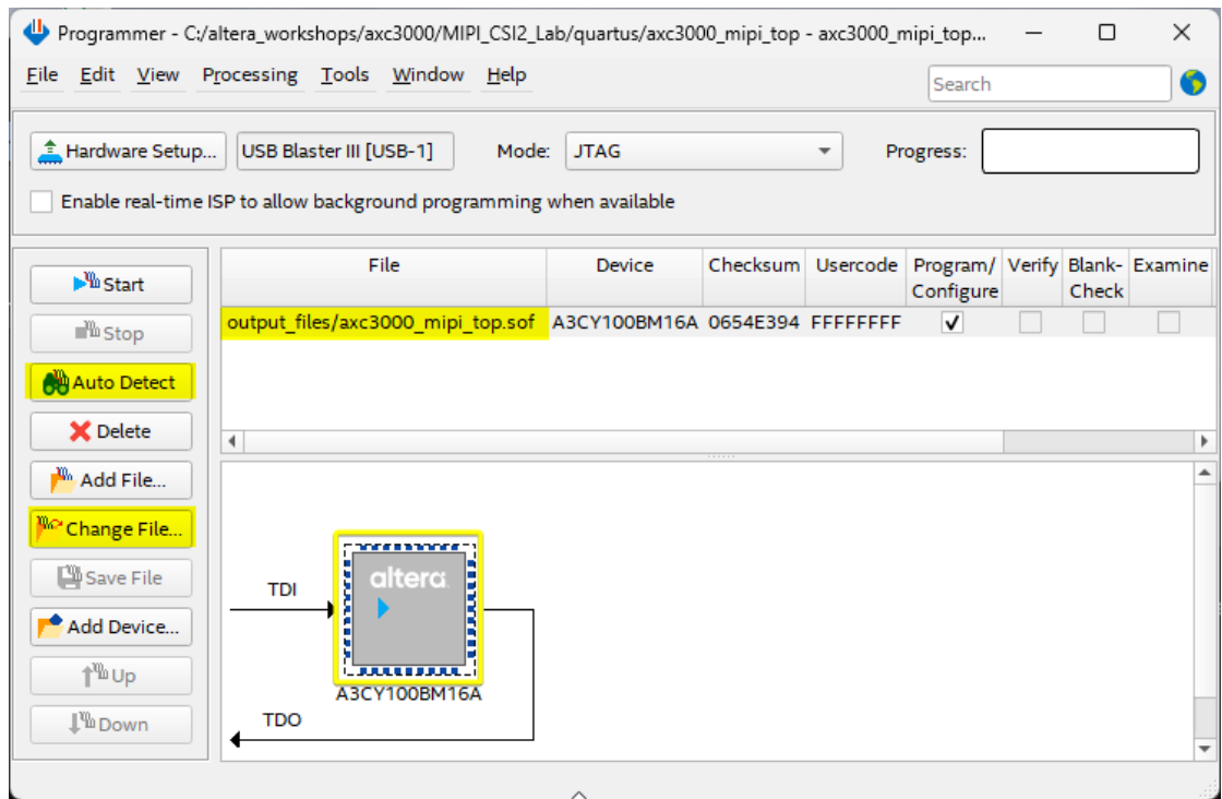
Figure 8-6 : Detect device and assign .sof file
