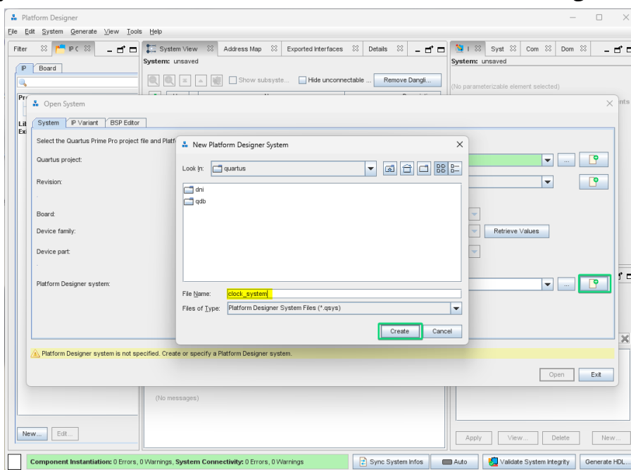
Figure 6-11: Create Platform Designer subsystem
