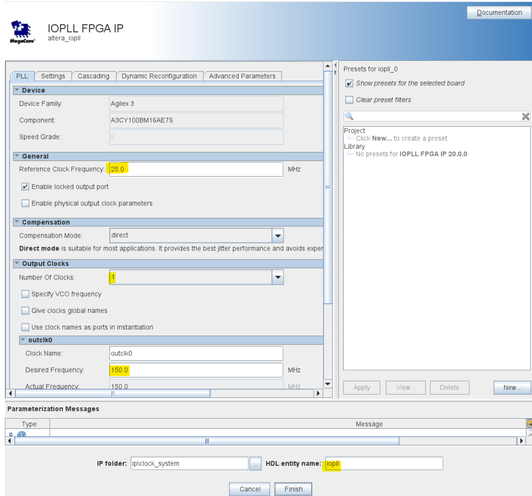
Figure 6-14: iopll Set up
