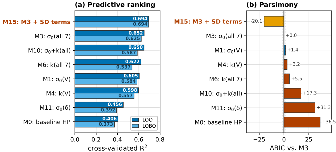
Family 3 Hall-Petch hierarchy for yield strength. Negative \Delta BIC favours the model over M3.
